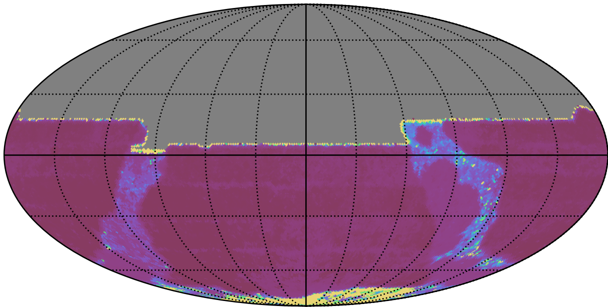
ddf_loaded_half_fl1_v3.4_10yrs All sky y band: Median Inter-Night Gap
