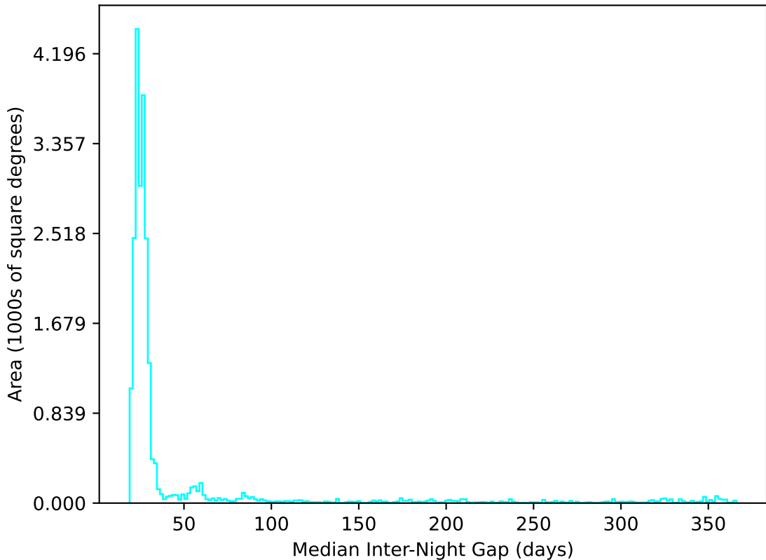
ddf_loaded_half_fl1_v3.4_10yrs All sky u band: Median Inter-Night Gap
