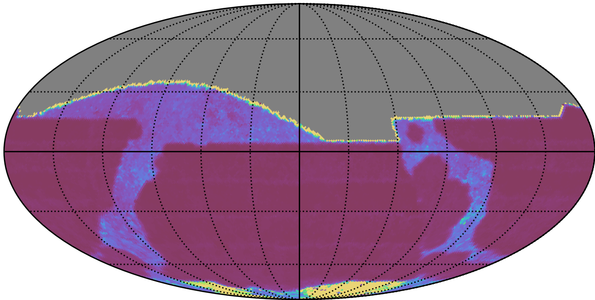
ddf_loaded_half_f11_v3.4_10yrs All sky r band: Median Inter-Night Gap
