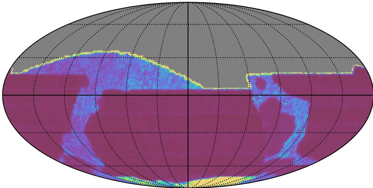
ddf_loaded_half_fl1_v3.4_10yrs All sky i band: Median Inter-Night Gap
