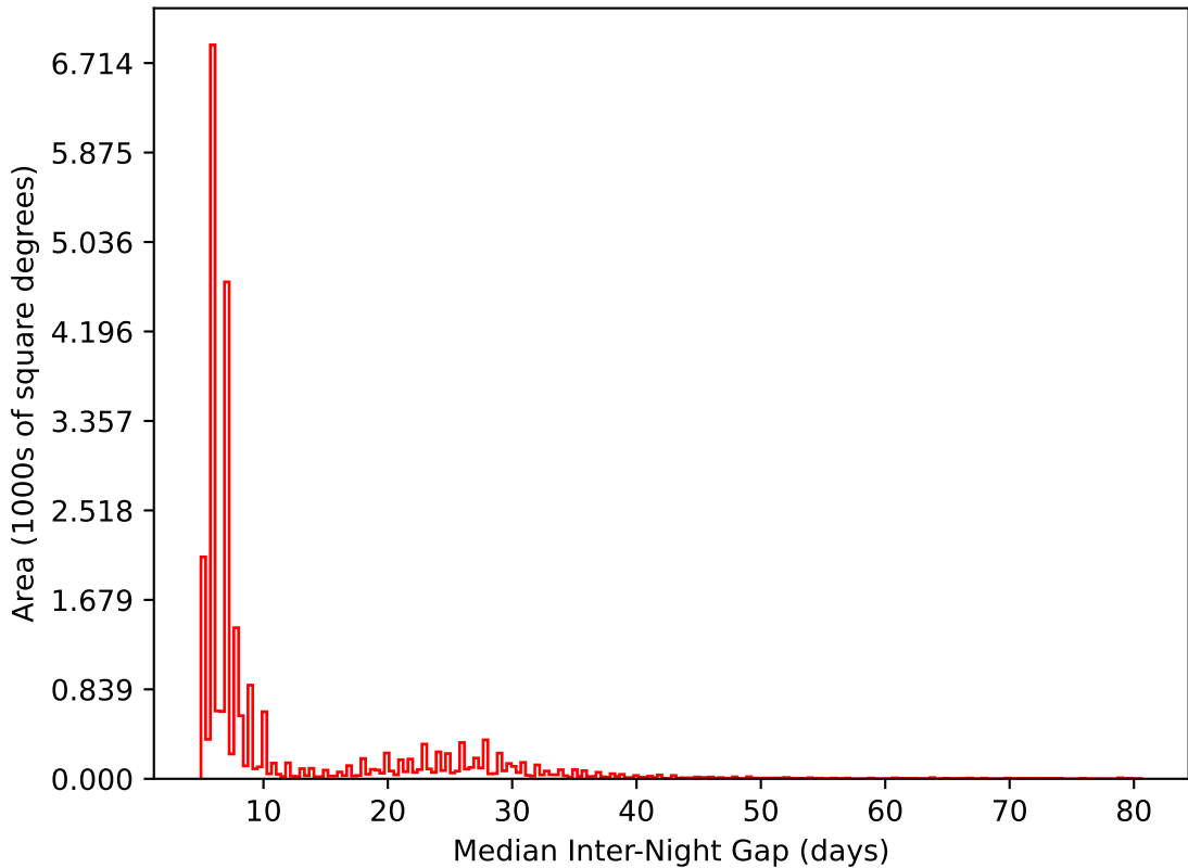
ddf_loaded_half_fl1_v3.4_10yrs All sky i band: Median Inter-Night Gap
