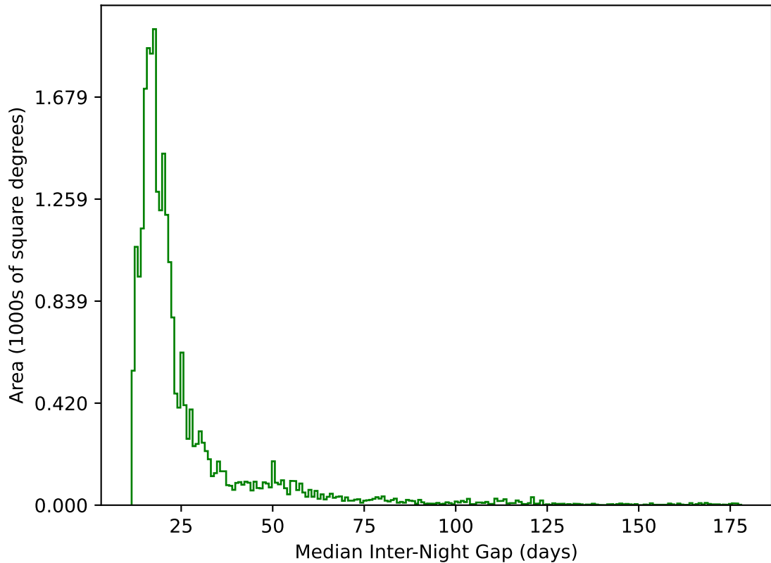
ddf_loaded_half_fl1_v3.4_10yrs All sky g band: Median Inter-Night Gap
