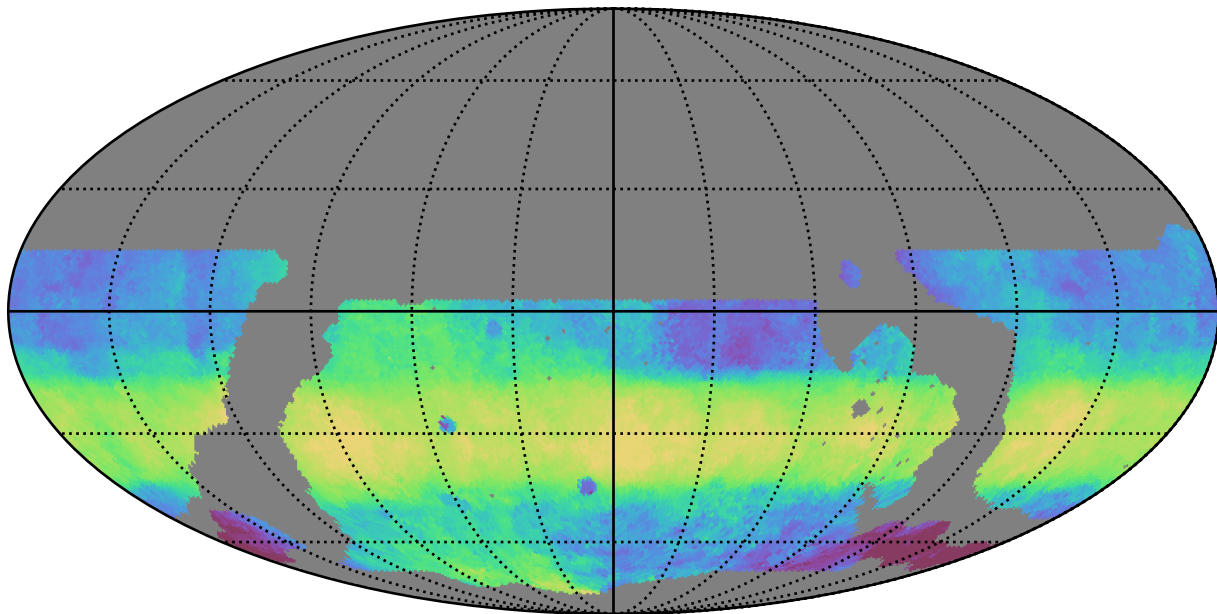
ddf_loaded_half_fl1_v3.4_10yrs WFD z band: Median HA
