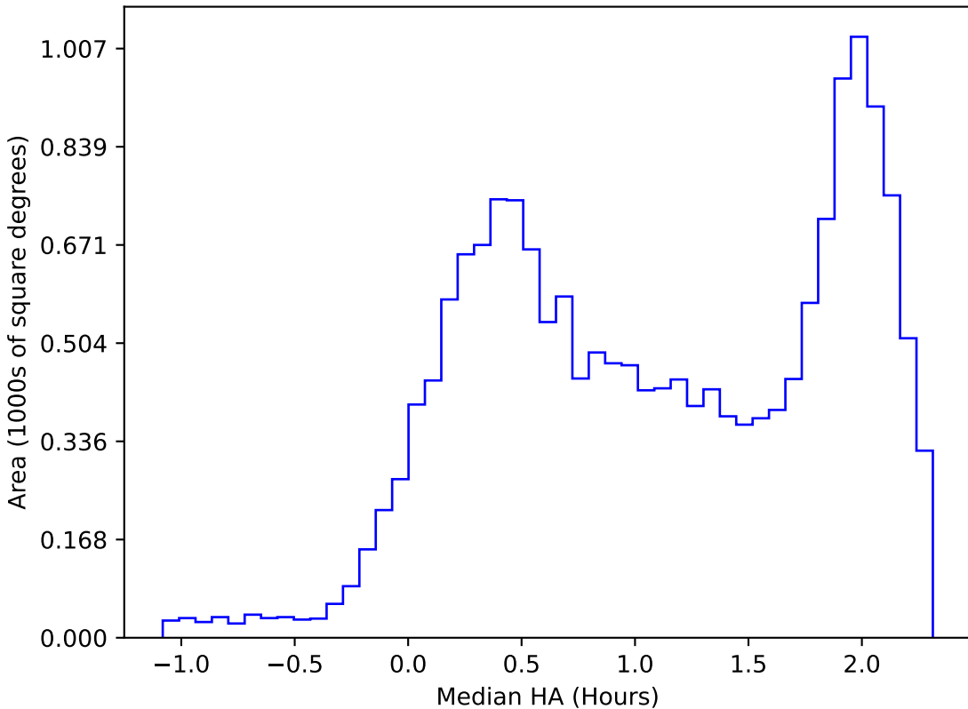
ddf_loaded_half_fl1_v3.4_10yrs WFD z band: Median HA
