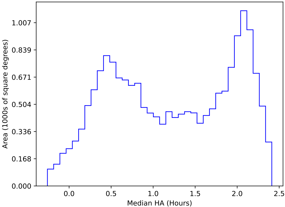
ddf_loaded_half_fl1_v3.4_10yrs WFD y band: Median HA
