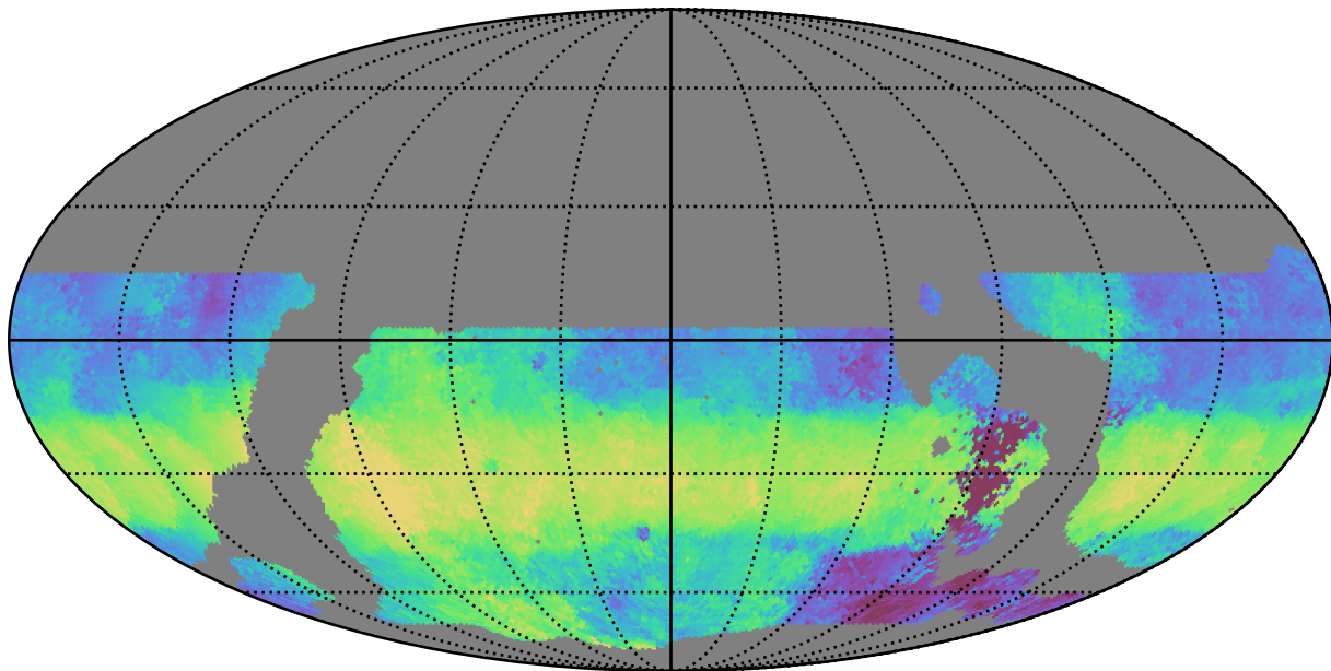
ddf_loaded_half_fl1_v3.4_10yrs WFD u band: Median HA
