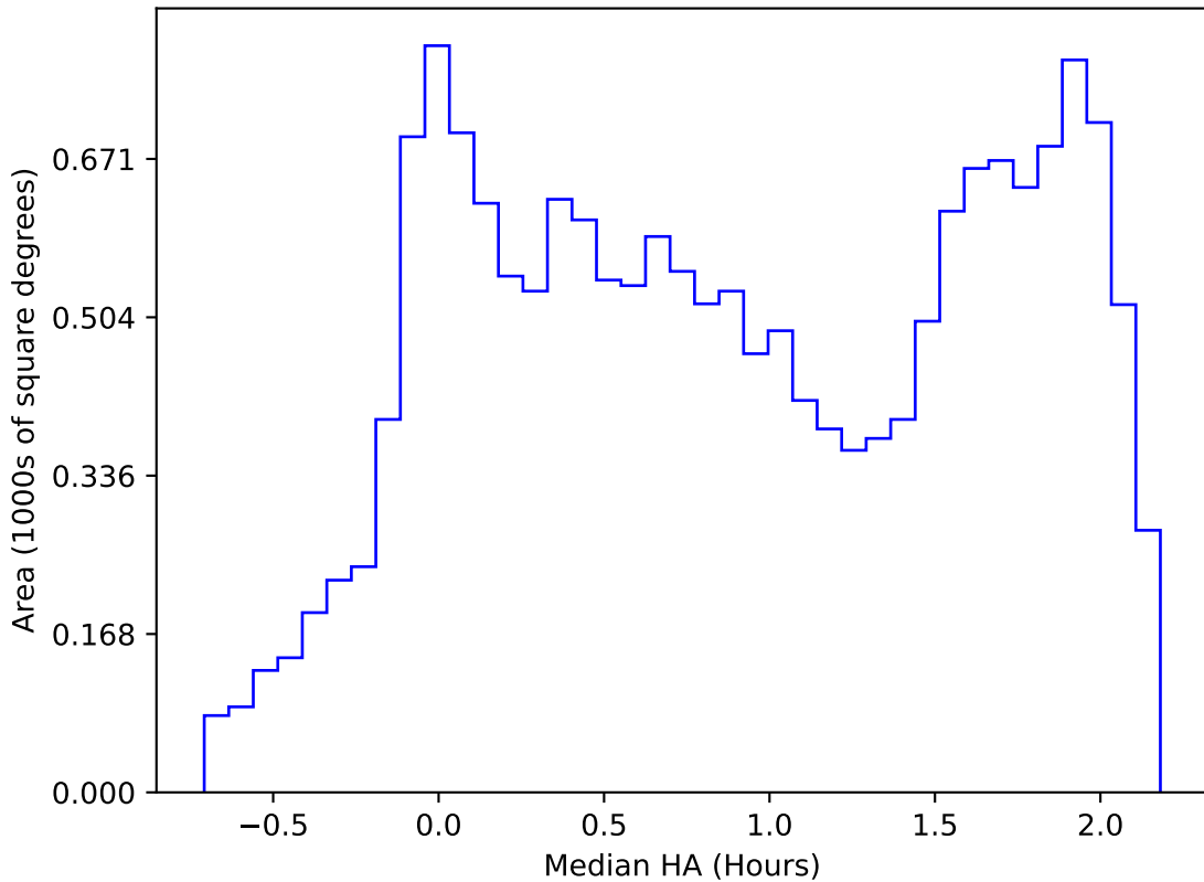
ddf_loaded_half_fl1_v3.4_10yrs WFD r band: Median HA
