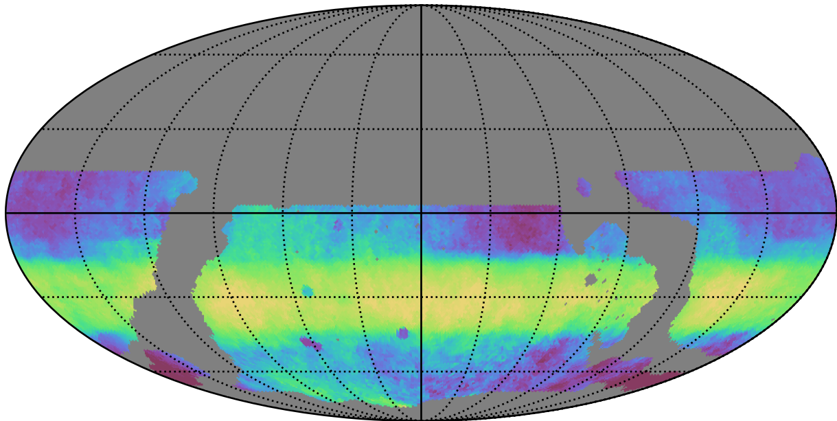
ddf_loaded_half_fl1_v3.4_10yrs WFD i band: Median HA
