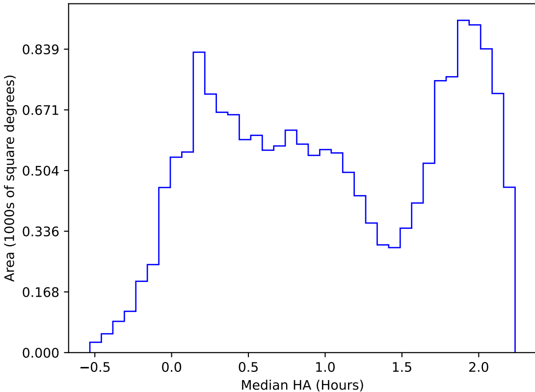
ddf_loaded_half_fl1_v3.4_10yrs WFD i band: Median HA
