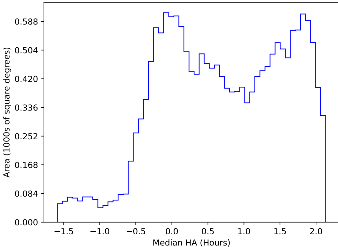
ddf_loaded_half_fl1_v3.4_10yrs WFD g band: Median HA
