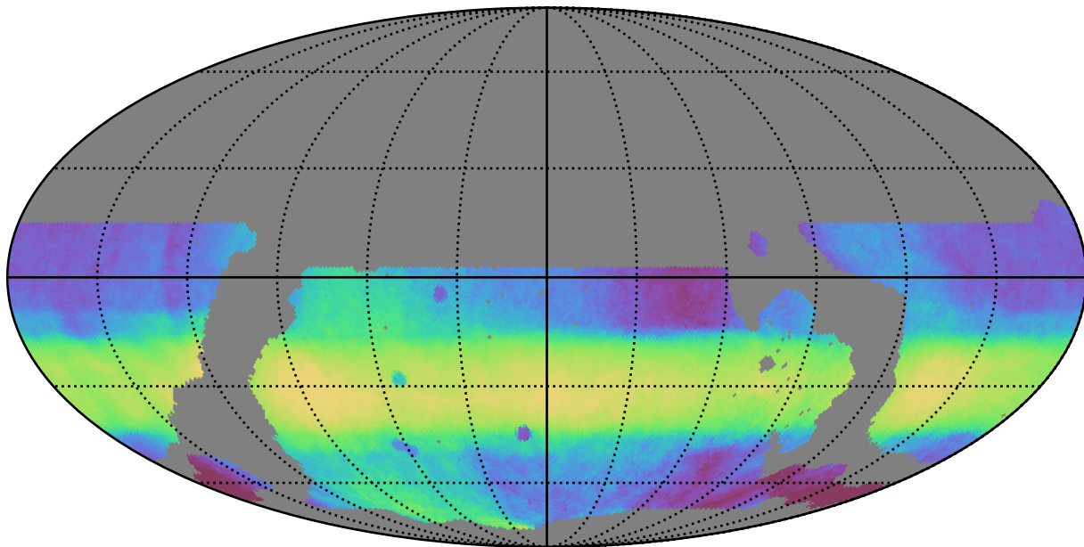
ddf_loaded_half_fl1_v3.4_10yrs WFD all bands: Median HA
