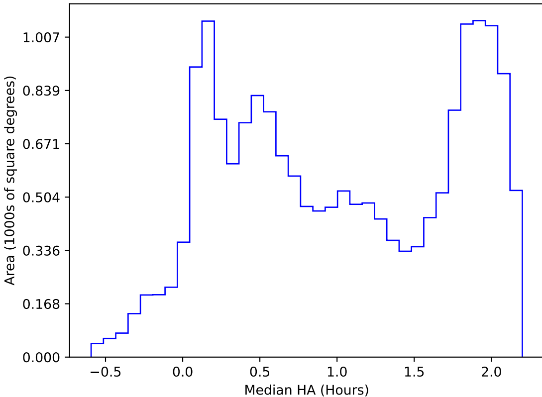
ddf_loaded_half_fl1_v3.4_10yrs WFD all bands: Median HA
