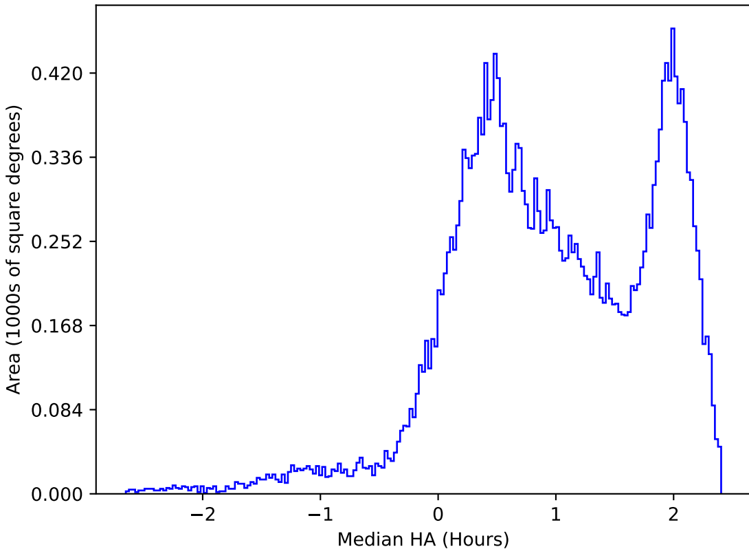
ddf_loaded_half_fl1_v3.4_10yrs All sky z band: Median HA
