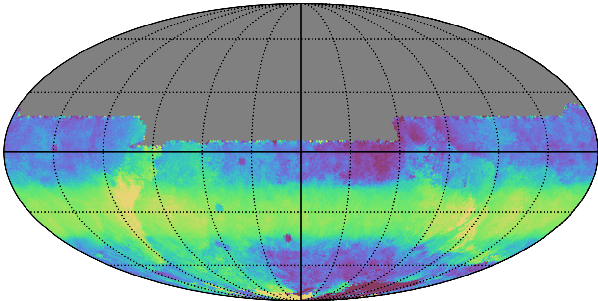
ddf_loaded_half_f11_v3.4_10yrs All sky y band: Median HA
