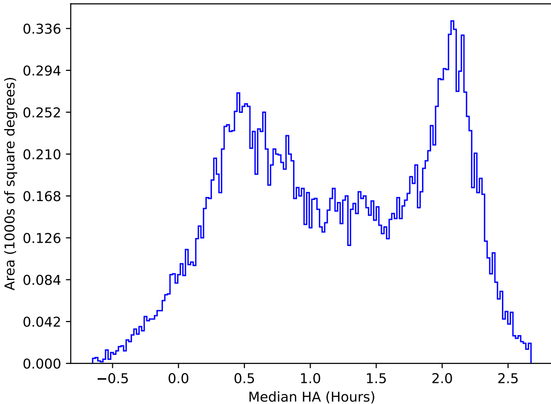
ddf_loaded_half_fl1_v3.4_10yrs All sky y band: Median HA
