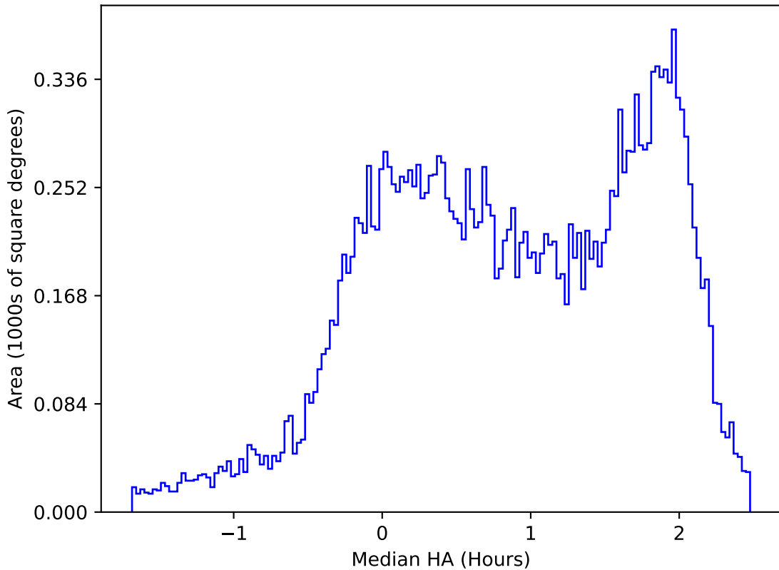
ddf_loaded_half_fl1_v3.4_10yrs All sky u band: Median HA
