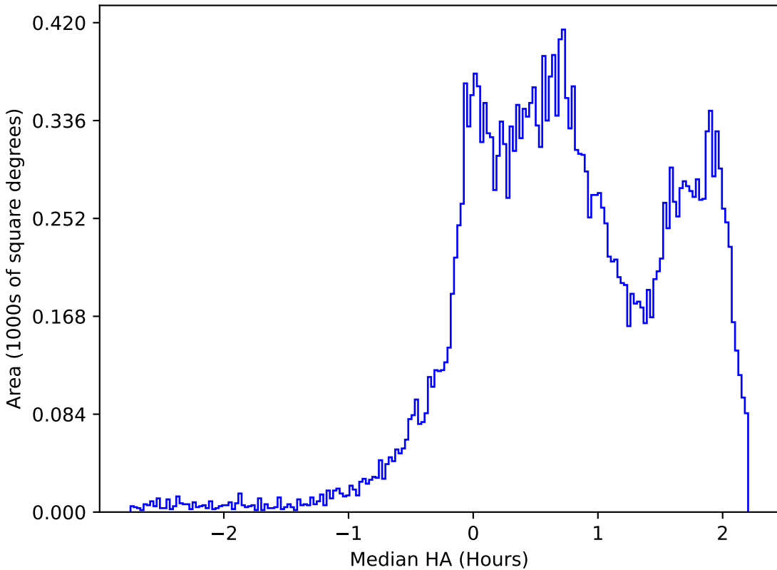
ddf_loaded_half_fl1_v3.4_10yrs All sky r band: Median HA
