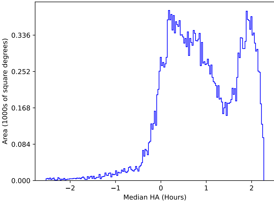
ddf_loaded_half_fl1_v3.4_10yrs All sky i band: Median HA
