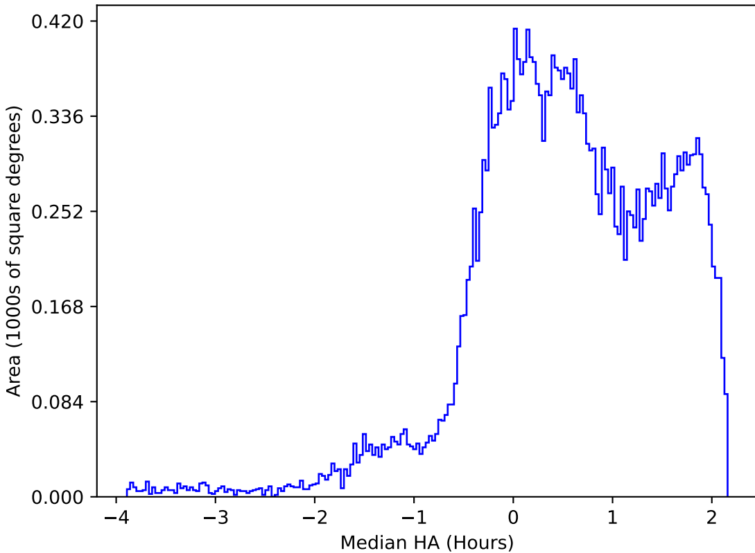
ddf_loaded_half_fl1_v3.4_10yrs All sky g band: Median HA
