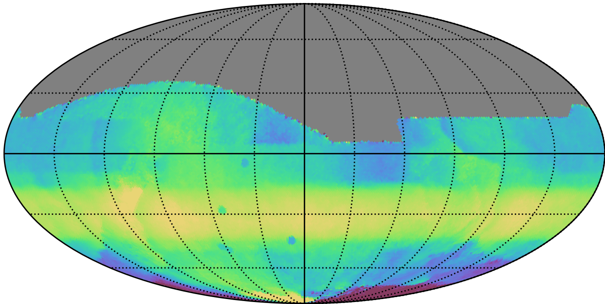
ddf_loaded_half_fl1_v3.4_10yrs All sky all bands: Median HA
