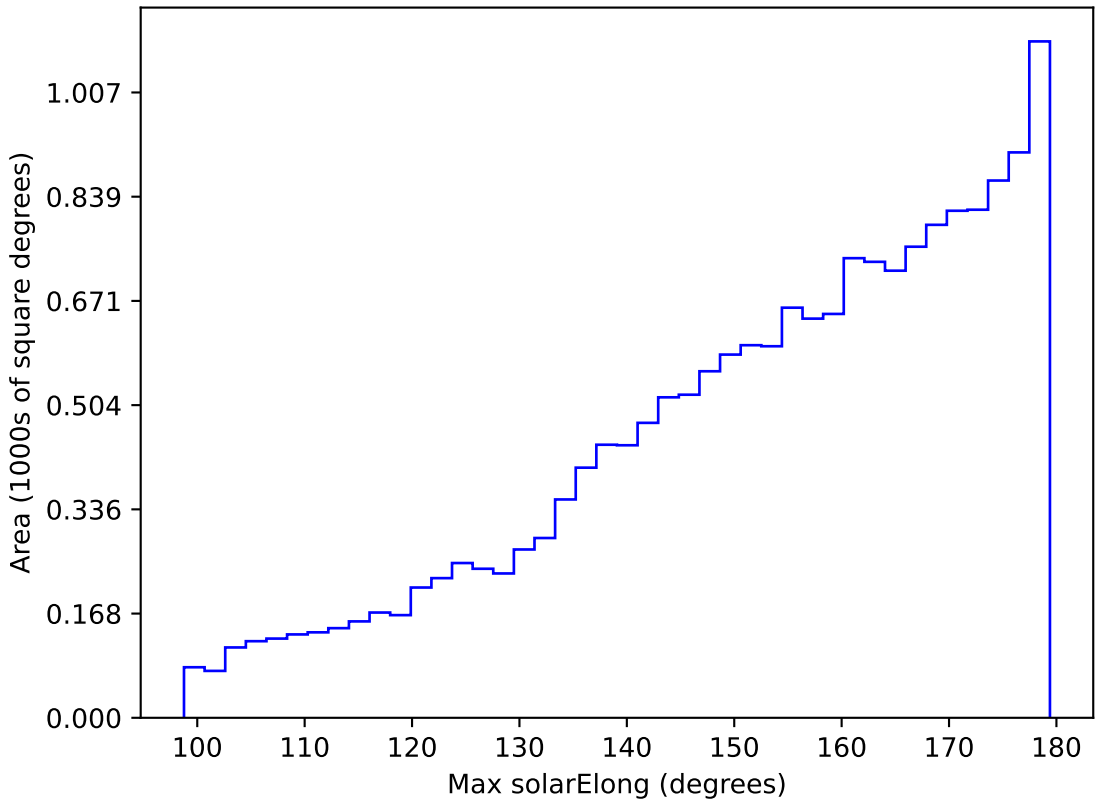
ddf_loaded_half_fl1_v3.4_10yrs WFD z band: Max solarElong
