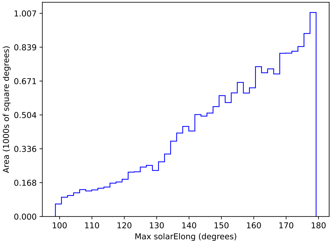
ddf_loaded_half_fl1_v3.4_10yrs WFD y band: Max solarElong
