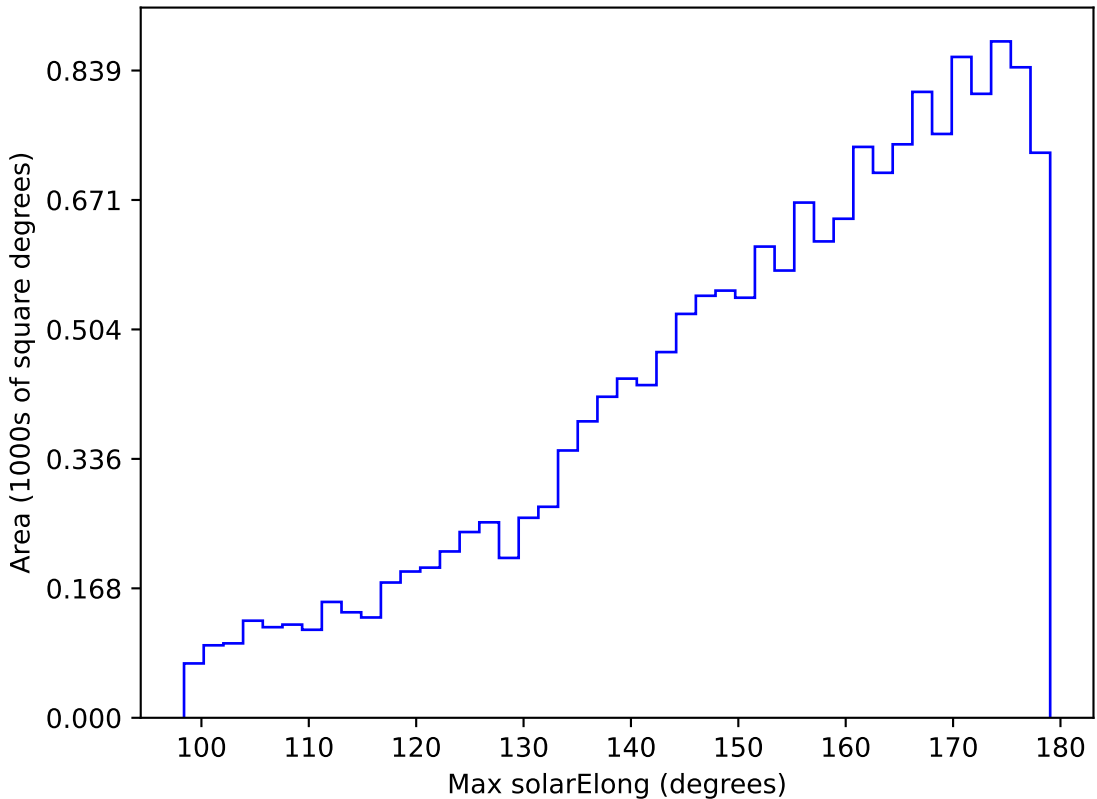
ddf_loaded_half_fl1_v3.4_10yrs WFD u band: Max solarElong
