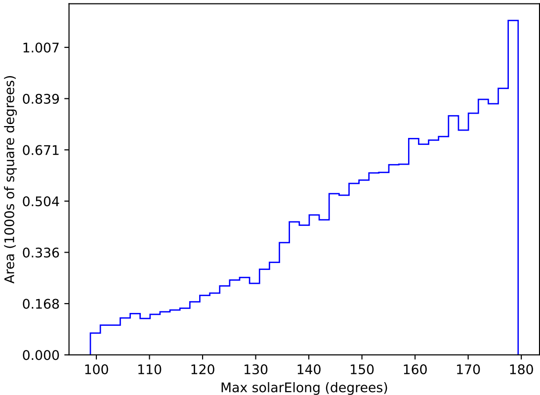
ddf_loaded_half_fl1_v3.4_10yrs WFD r band: Max solarElong
