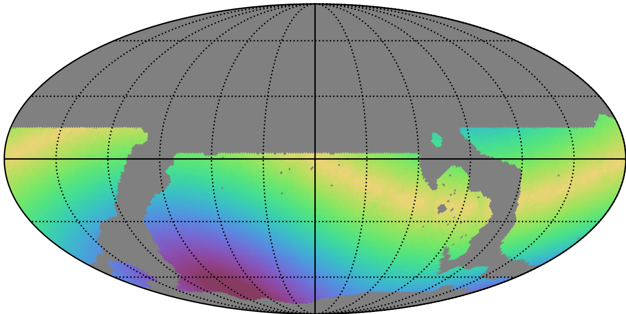
ddf_loaded_half_fl1_v3.4_10yrs WFD g band: Max solarElong
