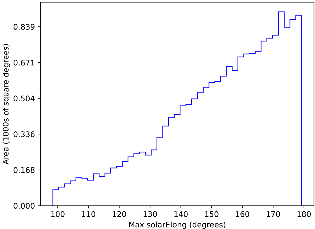
ddf_loaded_half_fl1_v3.4_10yrs WFD g band: Max solarElong
