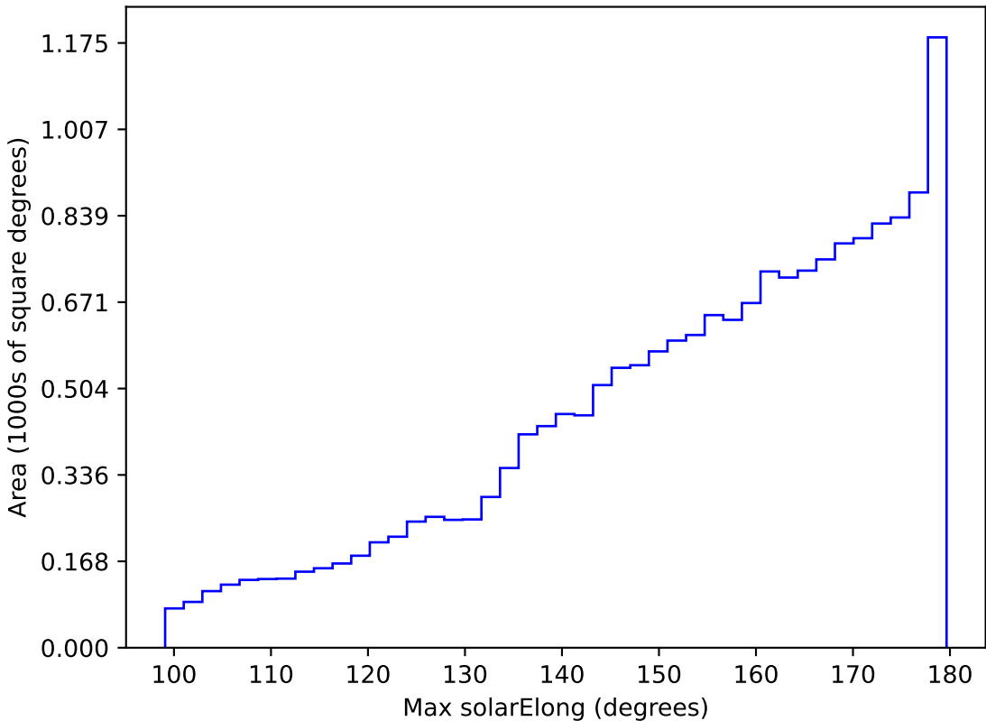
ddf_loaded_half_fl1_v3.4_10yrs WFD all bands: Max solarElong
