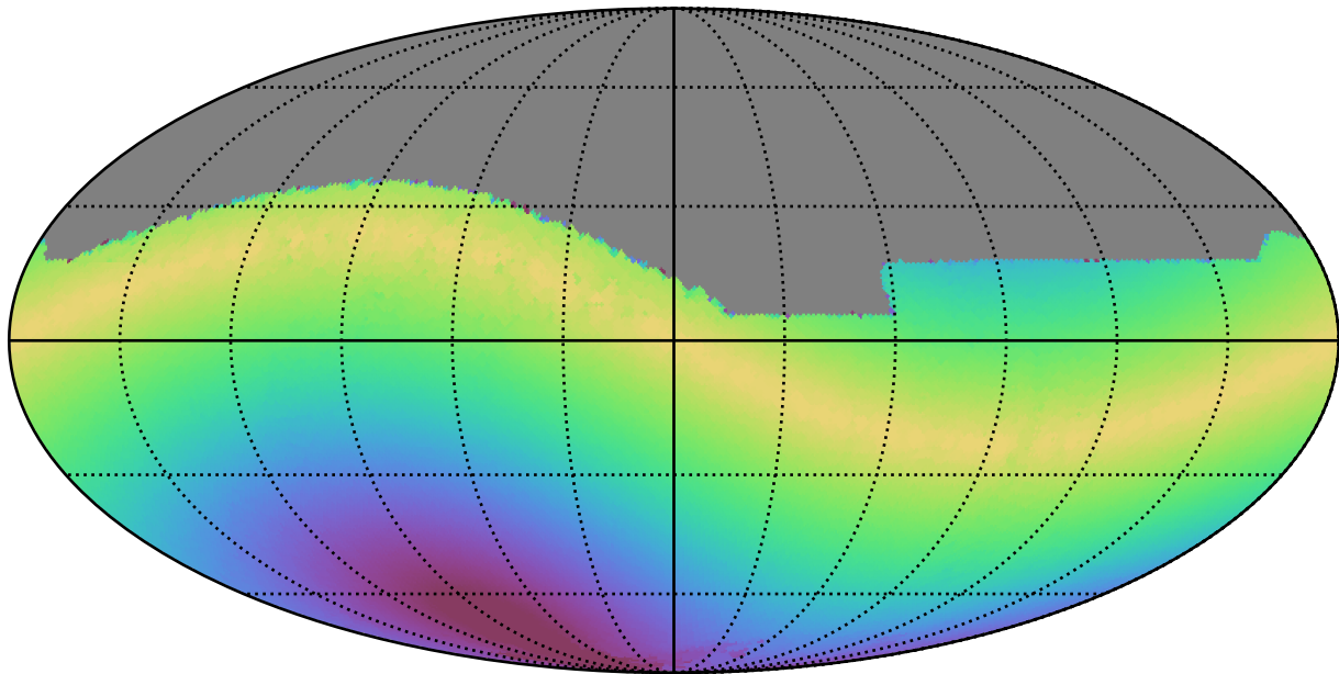
ddf_loaded_half_fl1_v3.4_10yrs All sky z band: Max solarElong
