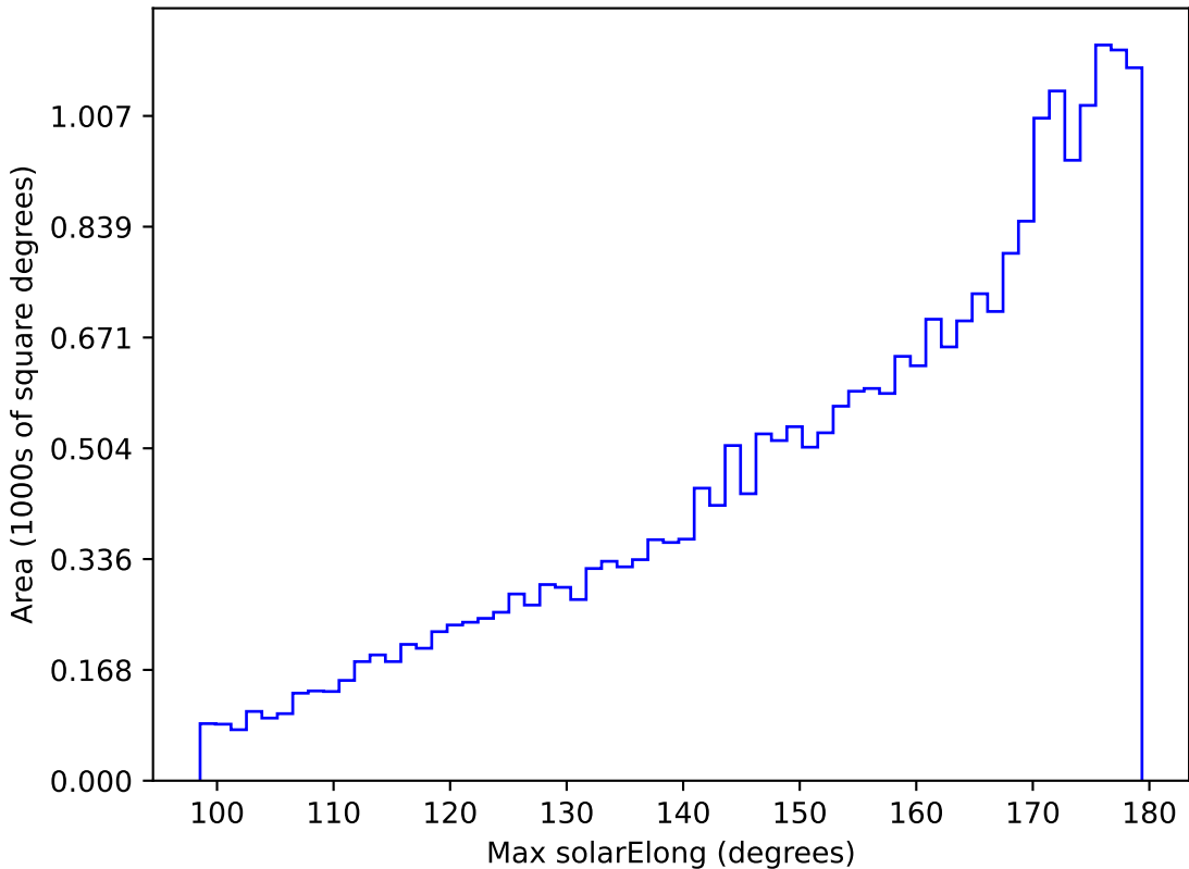
ddf_loaded_half_fl1_v3.4_10yrs All sky z band: Max solarElong
