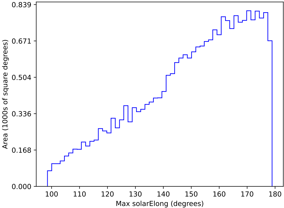
ddf_loaded_half_fl1_v3.4_10yrs All sky u band: Max solarElong
