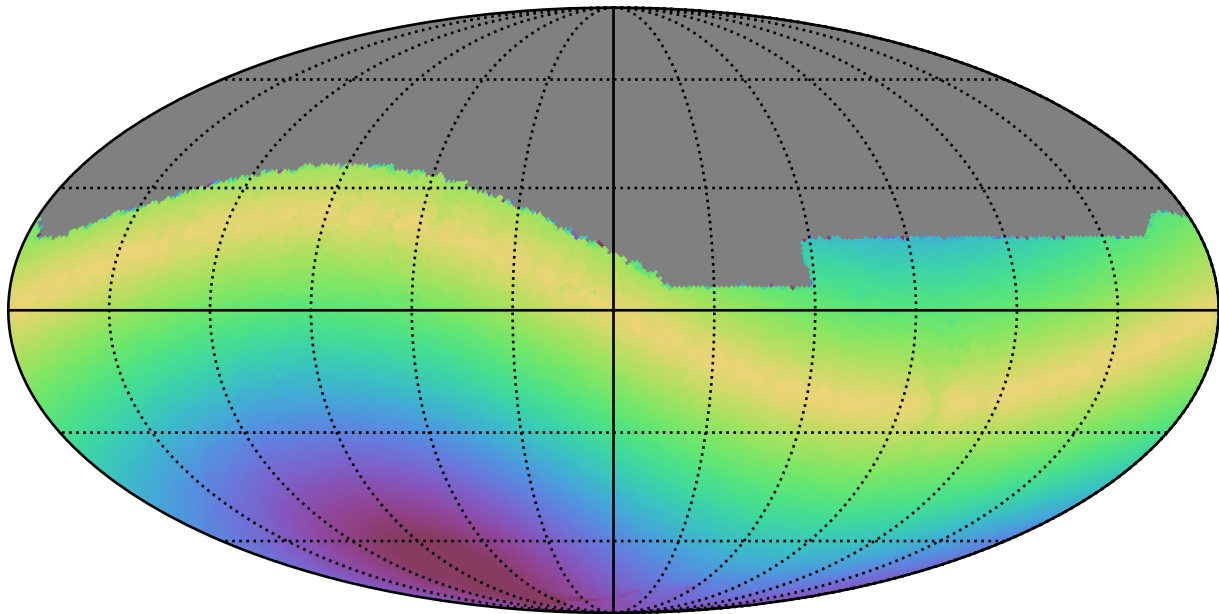
ddf_loaded_half_fl1_v3.4_10yrs All sky r band: Max solarElong
