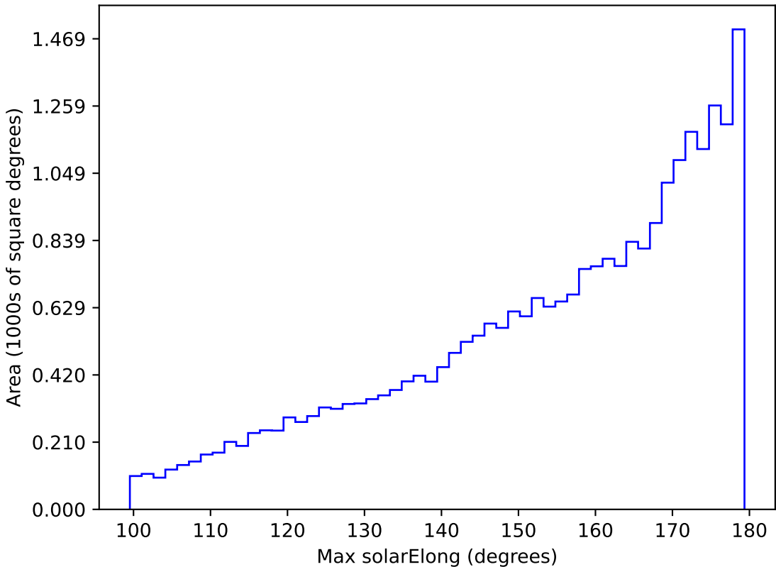
ddf_loaded_half_fl1_v3.4_10yrs All sky r band: Max solarElong
