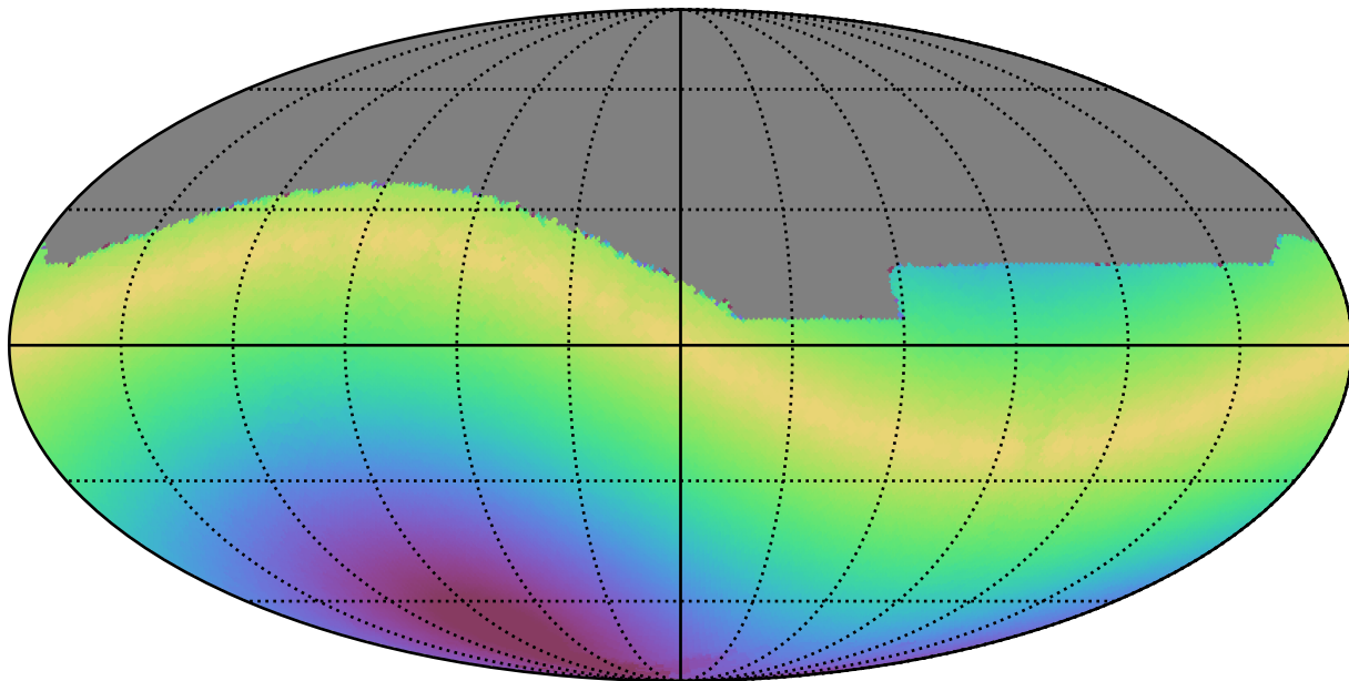
ddf_loaded_half_fl1_v3.4_10yrs All sky i band: Max solarElong
