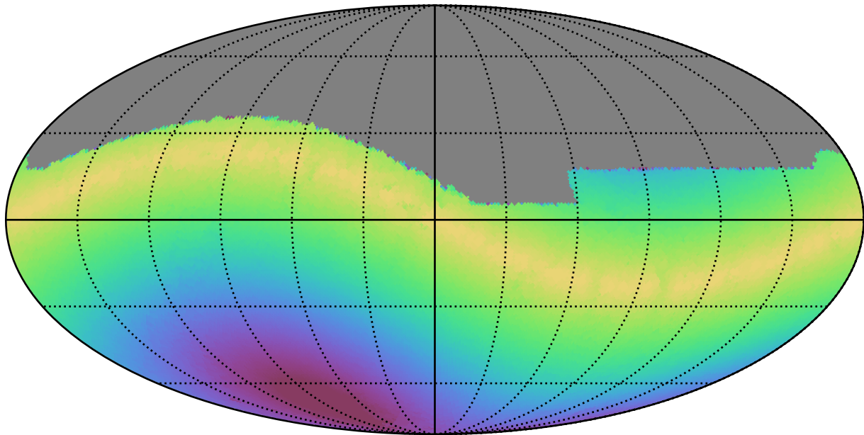
ddf_loaded_half_fl1_v3.4_10yrs All sky g band: Max solarElong
