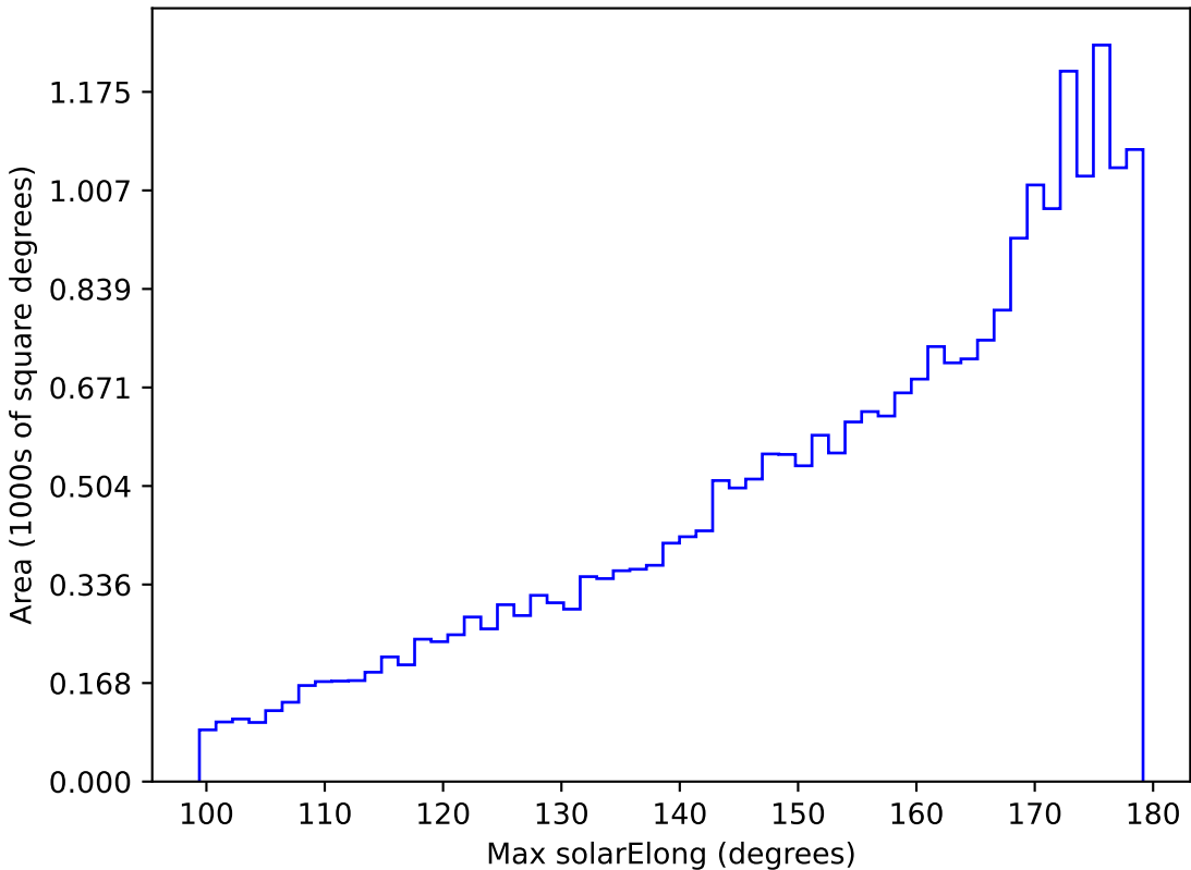
ddf_loaded_half_fl1_v3.4_10yrs All sky g band: Max solarElong
