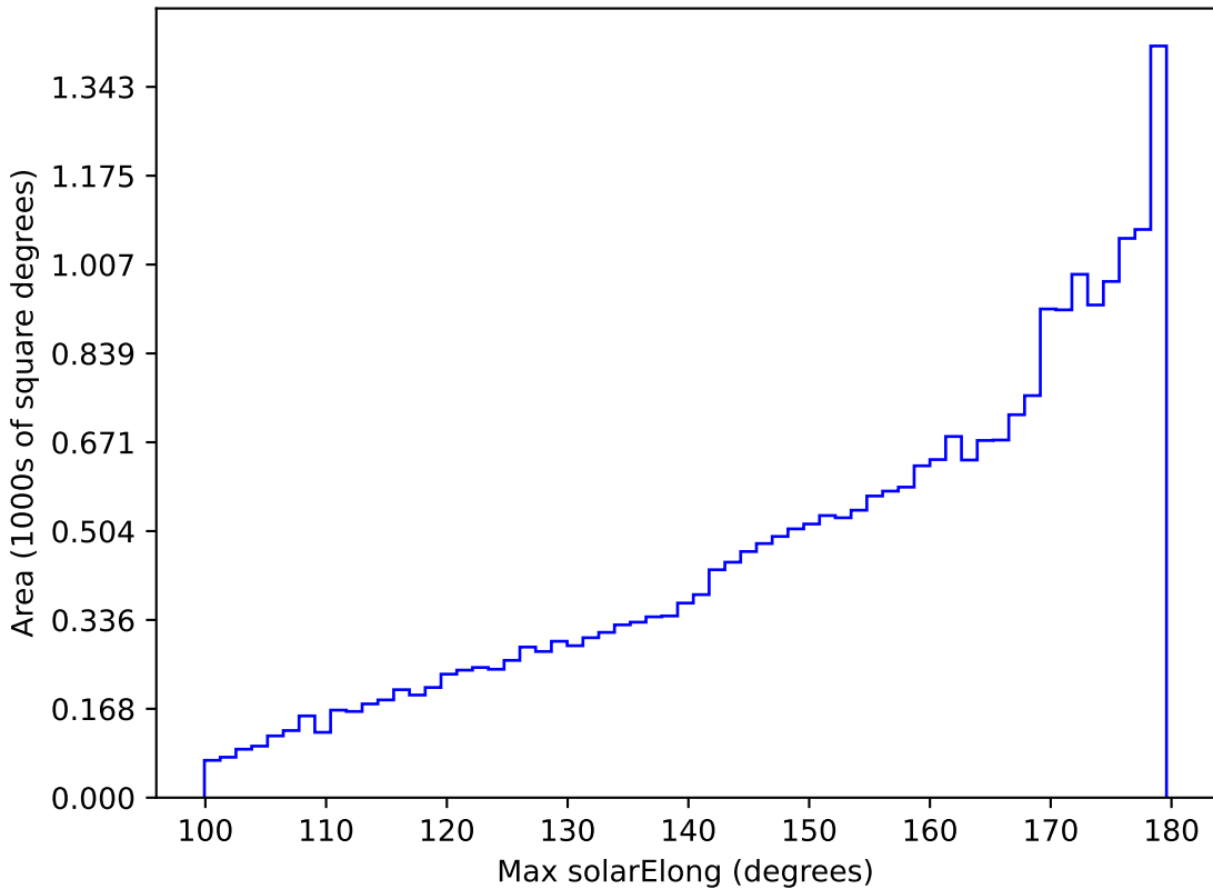
ddf_loaded_half_fl1_v3.4_10yrs All sky all bands: Max solarElong
