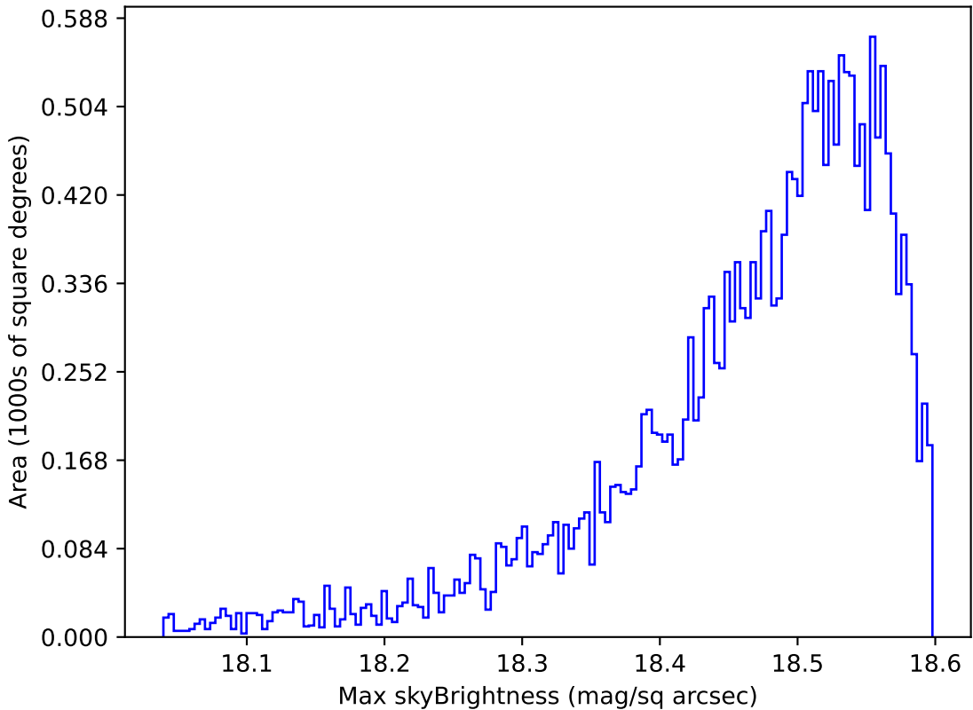
ddf_loaded_half_fl1_v3.4_10yrs Yr 1 y band: Max skyBrightness
