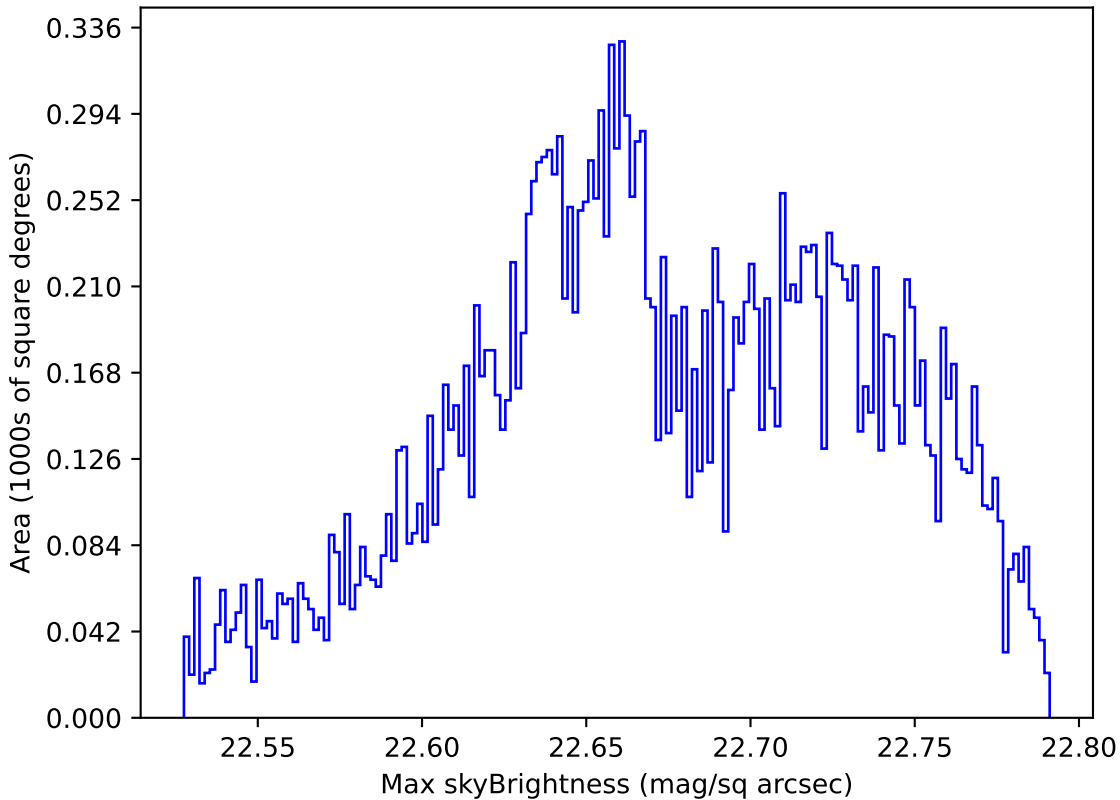
ddf_loaded_half_fl1_v3.4_10yrs Yr 1 u band: Max skyBrightness
