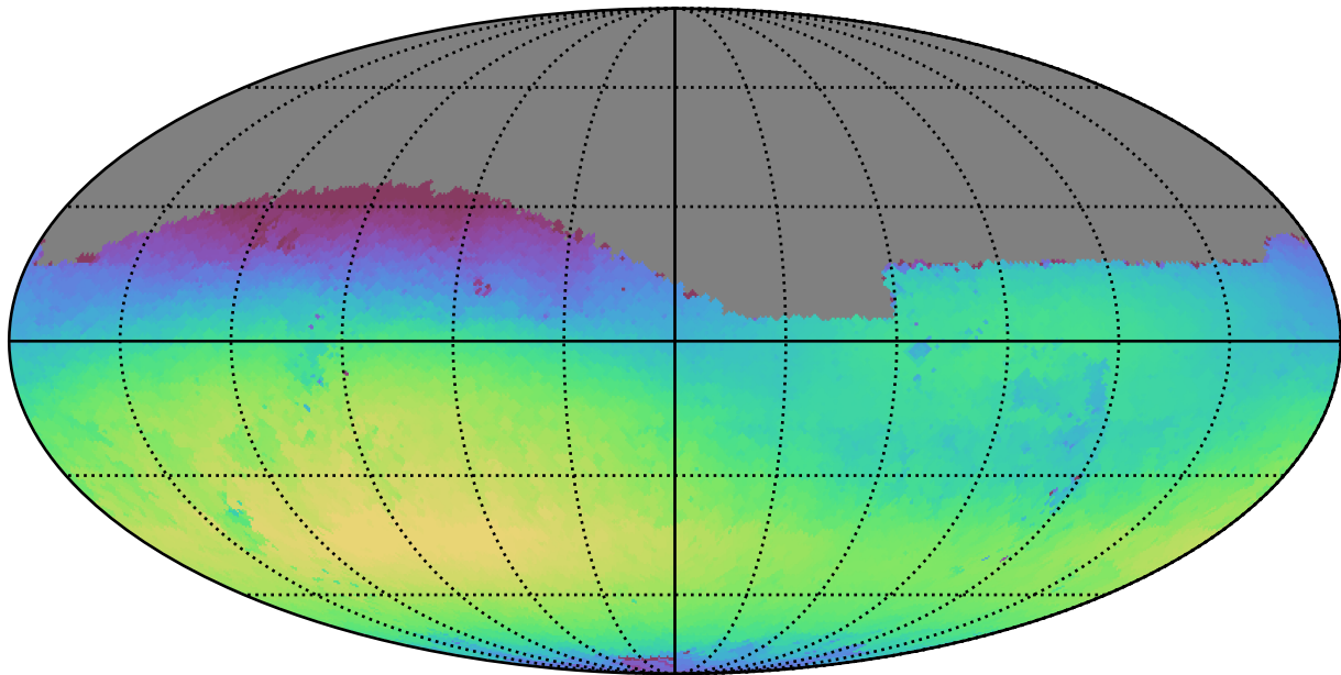
ddf_loaded_half_fl1_v3.4_10yrs Yr 1 r band: Max skyBrightness
