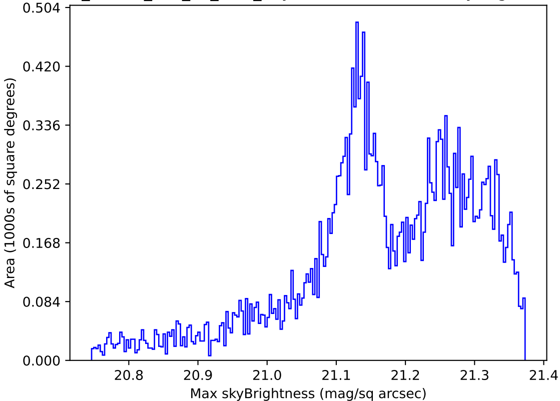
ddf_loaded_half_fl1_v3.4_10yrs Yr 1 r band: Max skyBrightness
