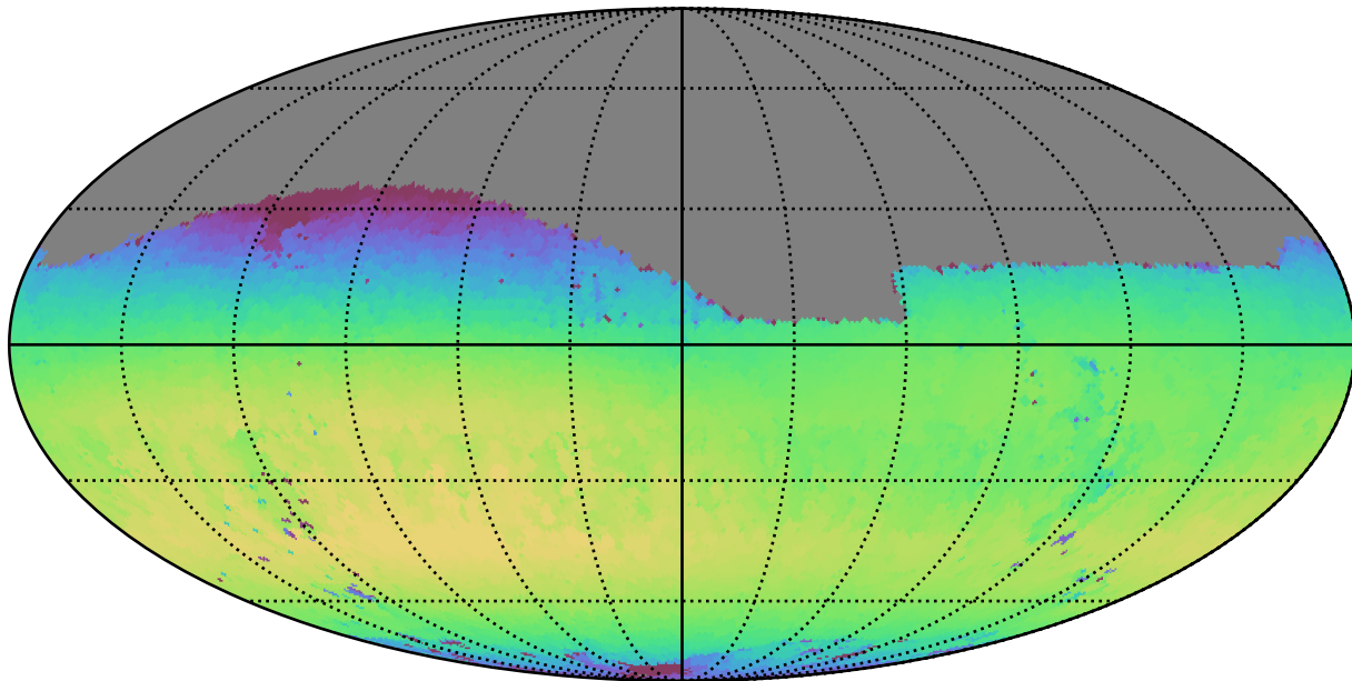
ddf_loaded_half_fl1_v3.4_10yrs Yr 1 i band: Max skyBrightness
