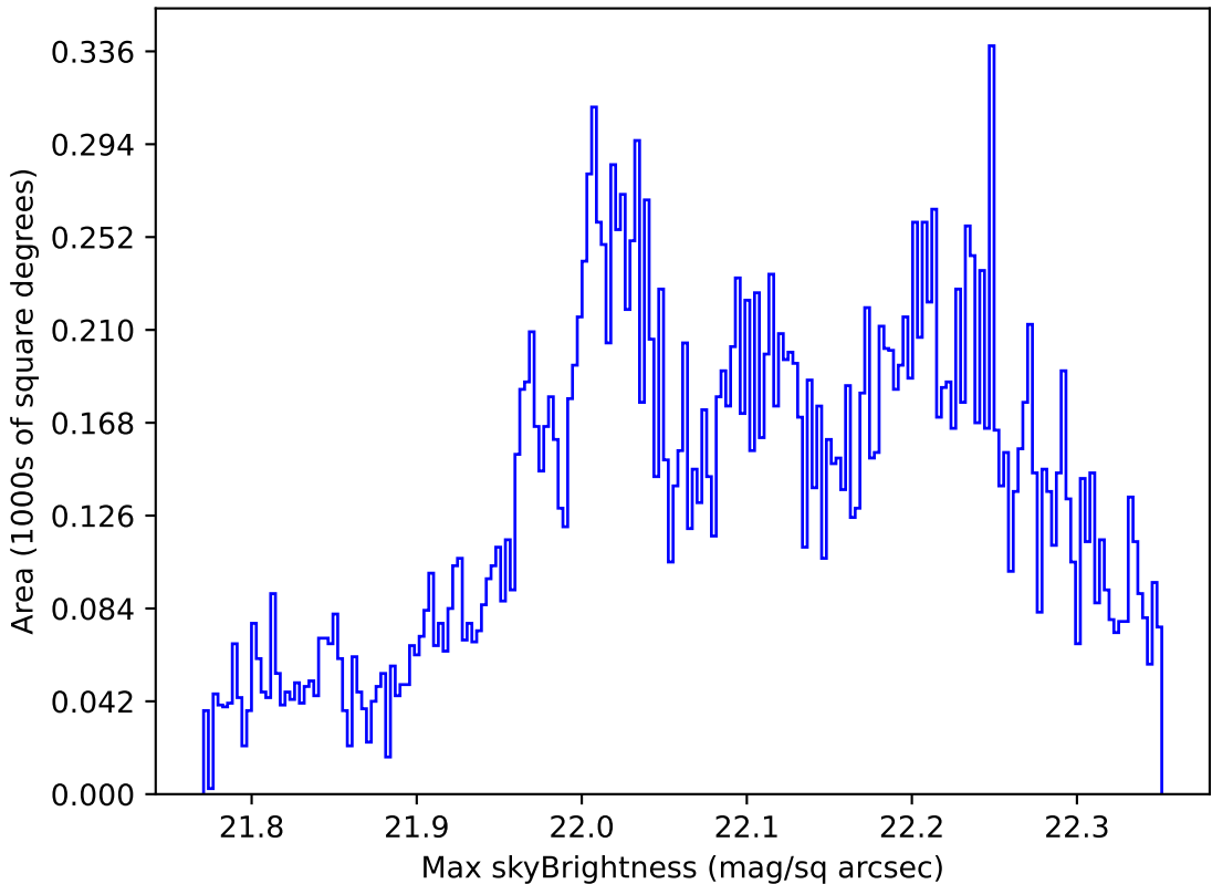
ddf_loaded_half_fl1_v3.4_10yrs Yr 1 g band: Max skyBrightness
