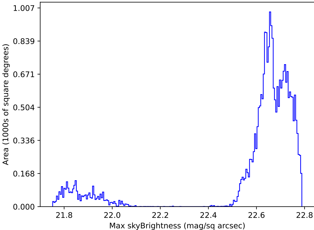
ddf_loaded_half_fl1_v3.4_10yrs Yr 1 all bands: Max skyBrightness
