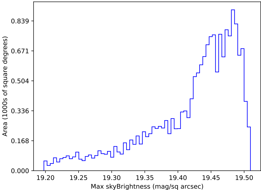
ddf_loaded_half_fl1_v3.4_10yrs WFD z band: Max skyBrightness
