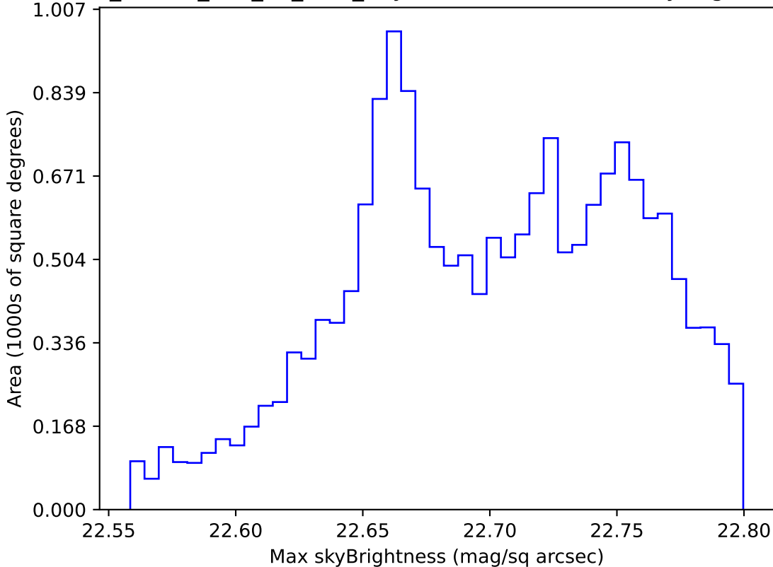
ddf_loaded_half_fl1_v3.4_10yrs WFD u band: Max skyBrightness
