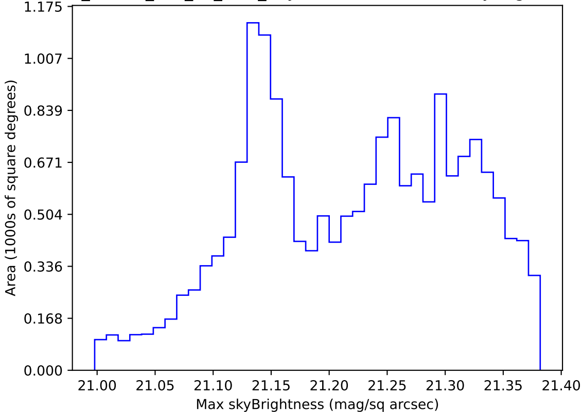
ddf_loaded_half_fl1_v3.4_10yrs WFD r band: Max skyBrightness
